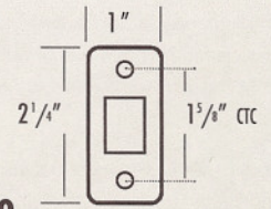
LFP.RO round latch face plate (available on request)
