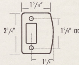
FLS.RO standard radius full lip strike (included with hardware)
