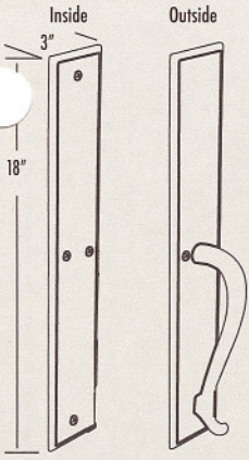
BZSQ.GE.18 Grip & Push (through bolt) 18 x 3" $ 710
