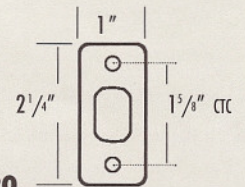
DFP.RO round deadbolt faceplate (available on request)
